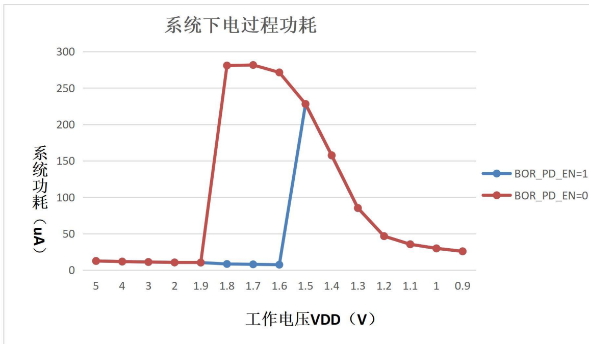
Figure 21-2 系统下电过程功耗
