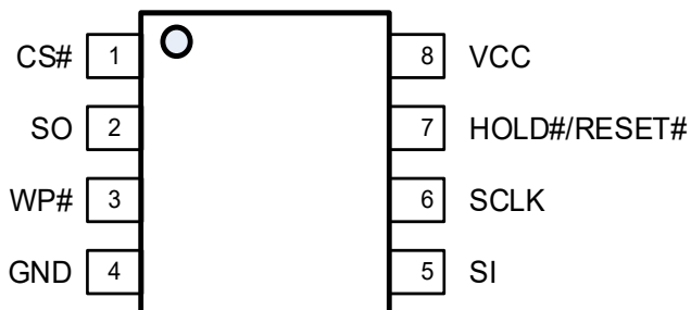
Figure 3-1 for SOP8 package
