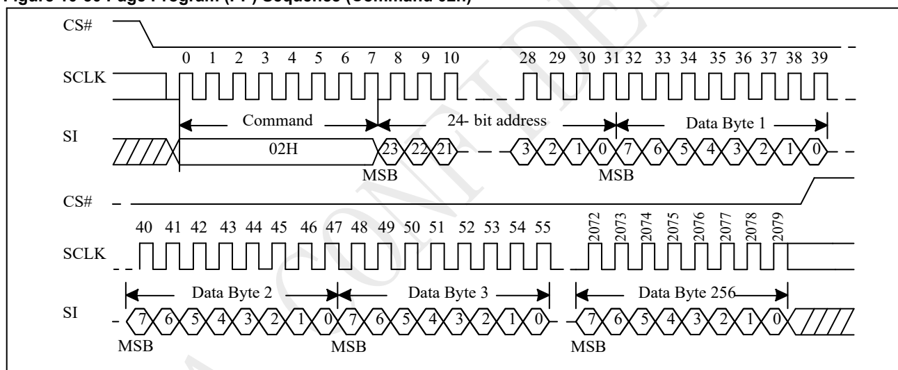
Figure 10-30 Page Program (PP) Sequence (Command 02h)
