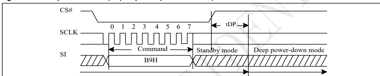
Figure 10-35 Deep Power-down (DP) Sequence (Command B9h)
