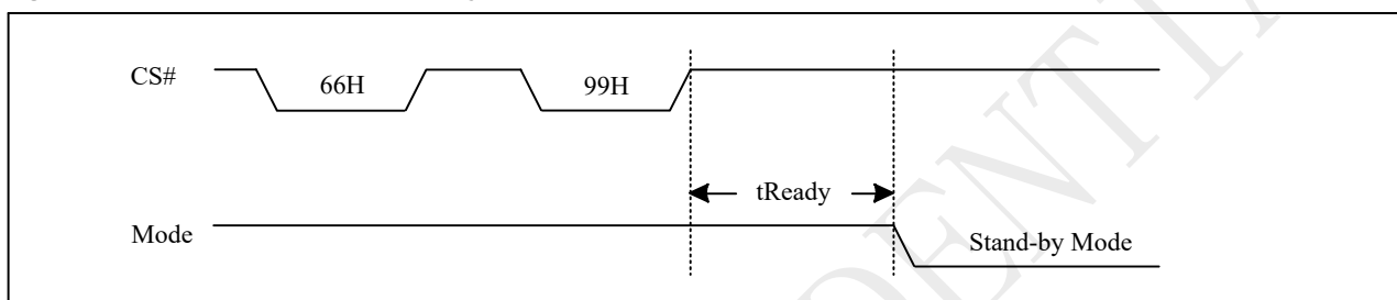
Figure 10-50a Reset Sequence
