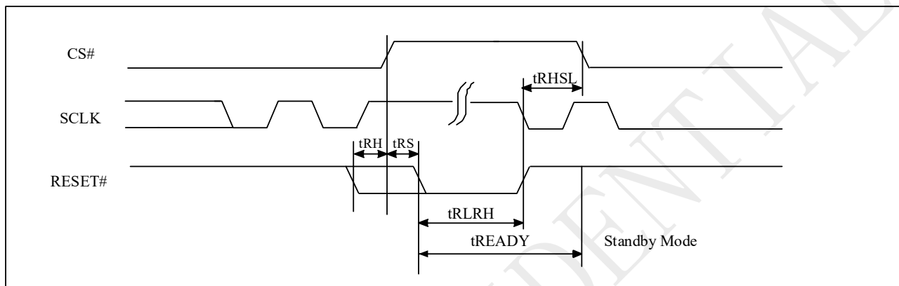
Figure 10-51 RESET Timing
