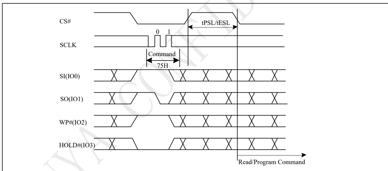
Figure 10-42a Suspend to Read/Program Latency (QPI)
