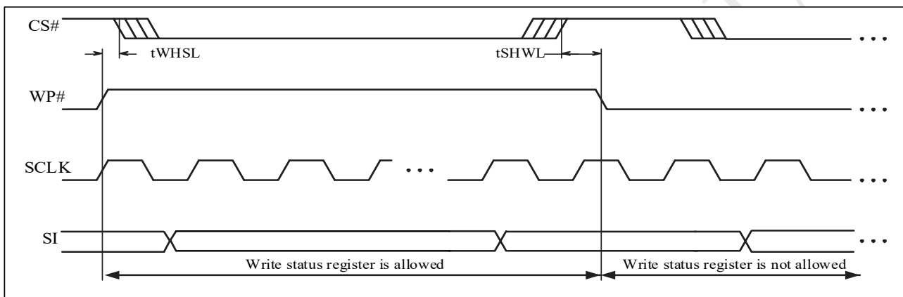
Figure 5-7 WP Timing
