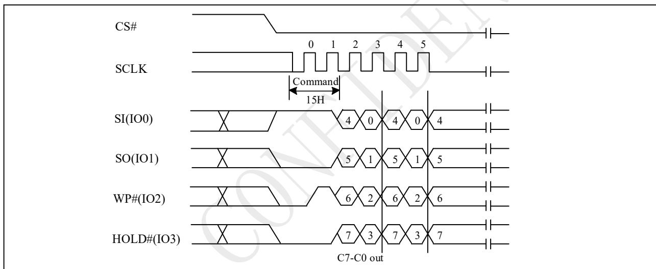
Figure 10-6a Read Status Register (RDCR) Sequence (QPI)
