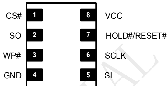
Figure 3-2 for WSON8 and USON8 package
