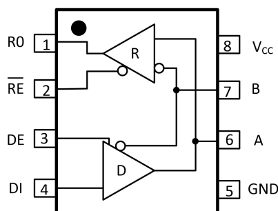
Pin Diagram
