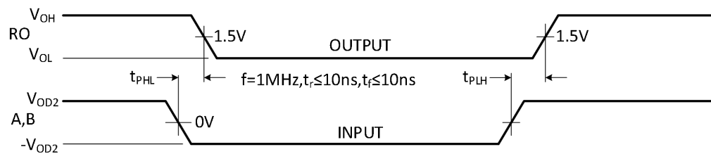
Figure 8. Receiver Propagation Delays
