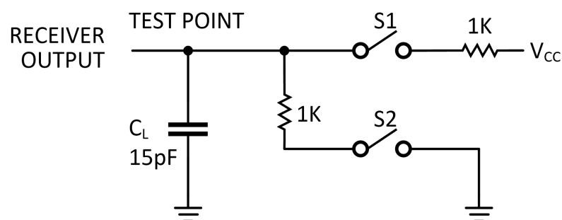
Figure 3. Receiver timing test load
