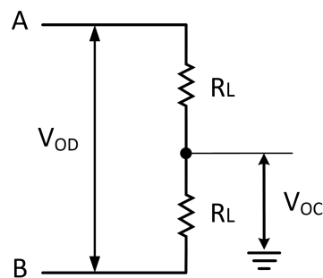
Figure 2. Driver DC test load
