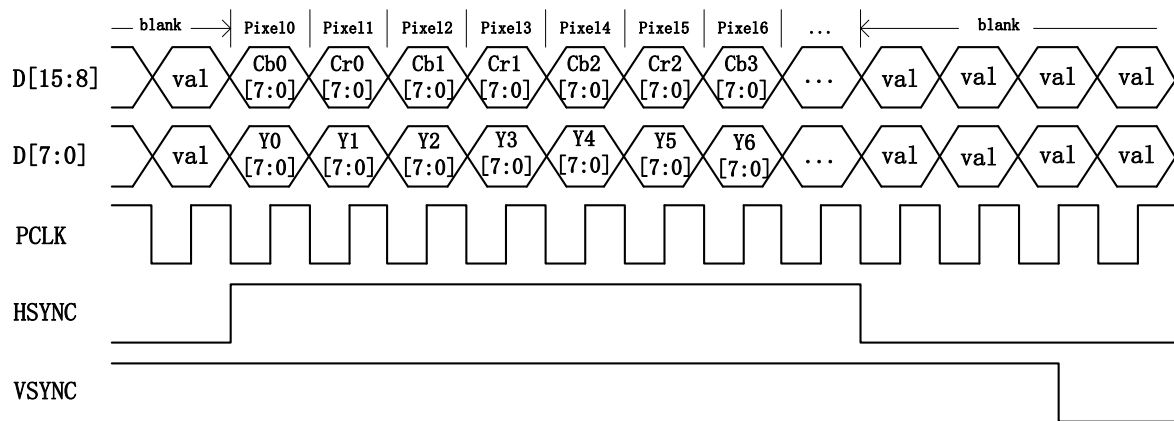
Figure 6-4. 16bit YCbCr4:2:2 with separate syncs Timing (clock rising edge sample.vsync valid = positive,hsync valid = positive)
