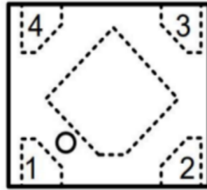
DFN1X1-4
