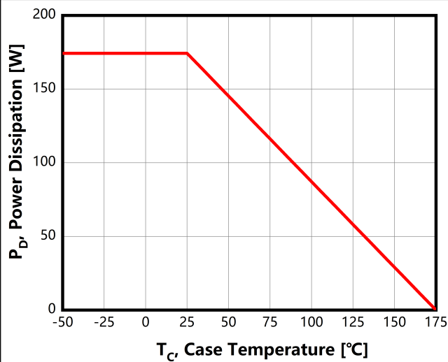
Figure 14. Maximum Power Dissipation Derating vs. Case Temperature
