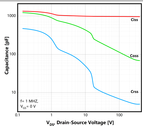
Figure 12. Capacitance Characteristics
