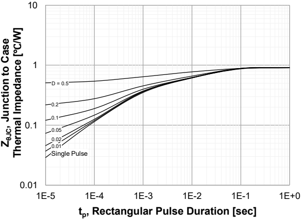
Figure 22. Transient Thermal Response Curve
