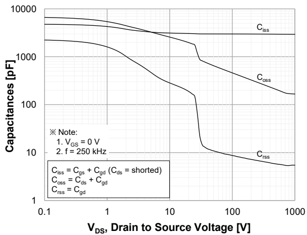
Figure 12. Capacitance Characteristics
