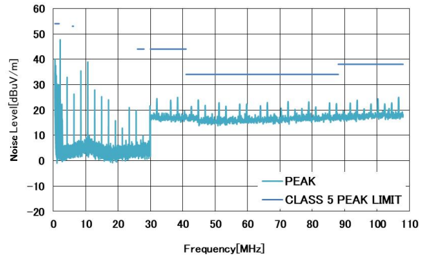
图 36. GM2500_DEMOZ CISPR25 Conducted Emission with Class 5 Peak Limits (Voltage Method)
