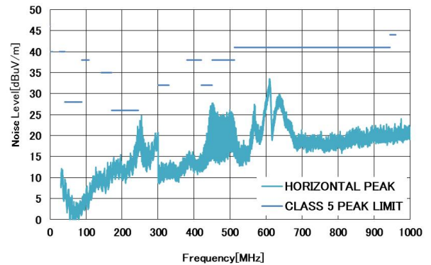
图 37. GM2500_DEMOZ CISPR25 Radiated Emission (Horizontal)
