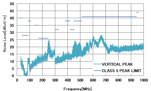
图 38. GM2500_DEMOZ CISPR25 Radiated Emission (Vertical)
