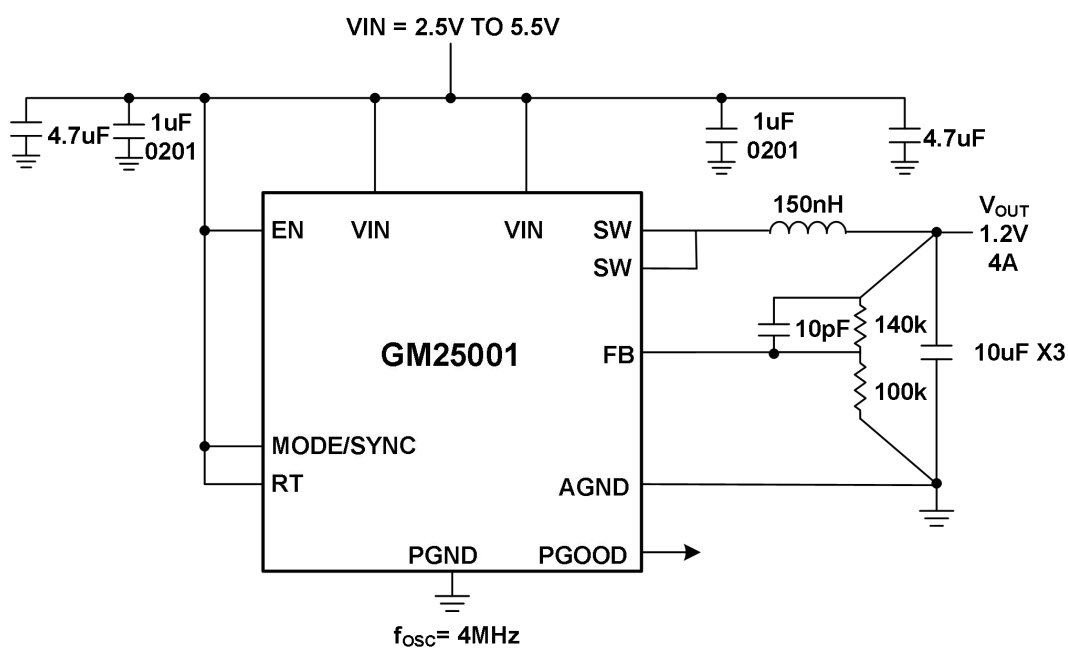
图 40. 4MHz, V IN =3.3V, V OUT =1.2V, I LOAD =4A
