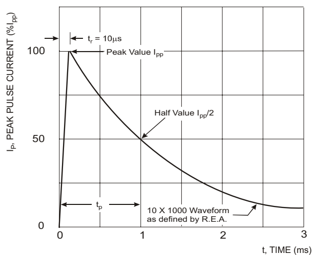
Fig. 4 Pulse Waveform
