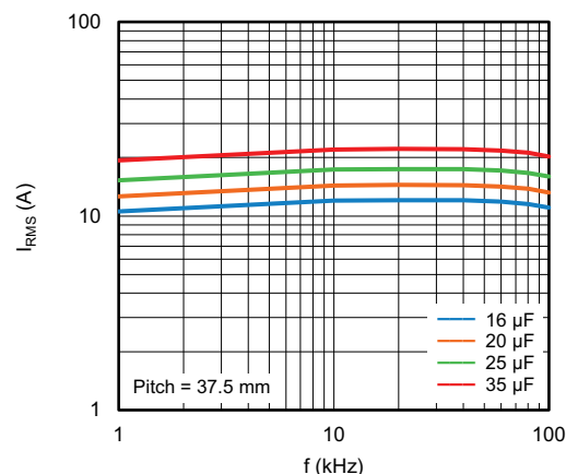
Maximum I_{\text{RMS}} current as function of frequency, based T_A + 85^\circ\text{C} , \Delta t = +15^\circ\text{C} (typical curve)
