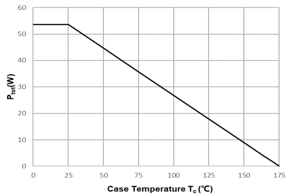
Fig12. Power Dissipation vs. Case temperature
