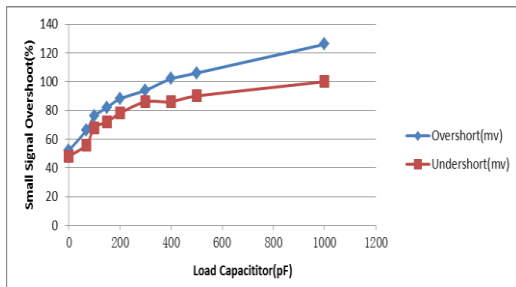
Overshoot (OS) vs Load Capacitance
