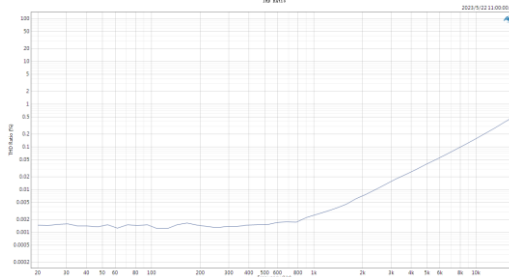
THD vs Frequency
