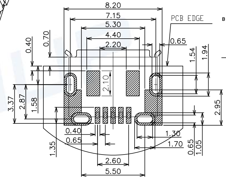
RECOMMENDED P.C.B LAYOUT COMPONENT SIDE(TOLERANCE ±0.05)
