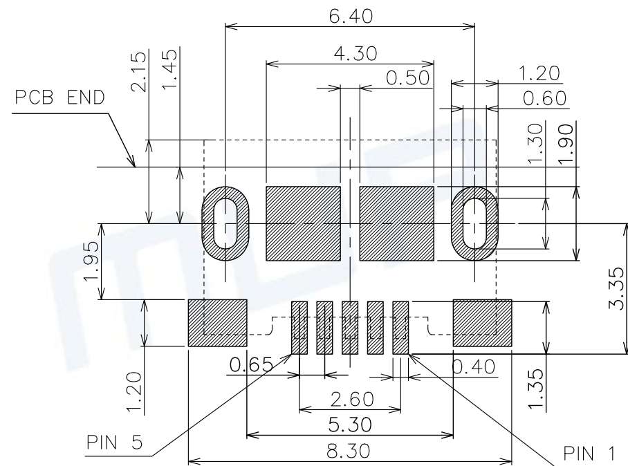
RECOMMENDED P.C.B LAYOUT COMPONENT SIDE(TOLERANCE ±0.05)
