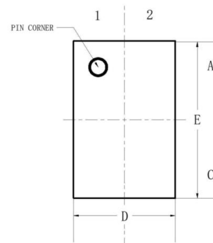
BOTTOM VIEW (BALL SIDE DOWN)
