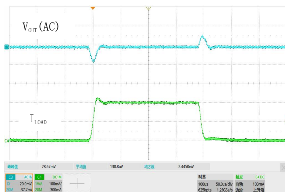
图 23. 负载瞬态响应, V_{IN}=4.3V , V_{OUT}=3.3V , I_{OUT}=1mA to 150mA
