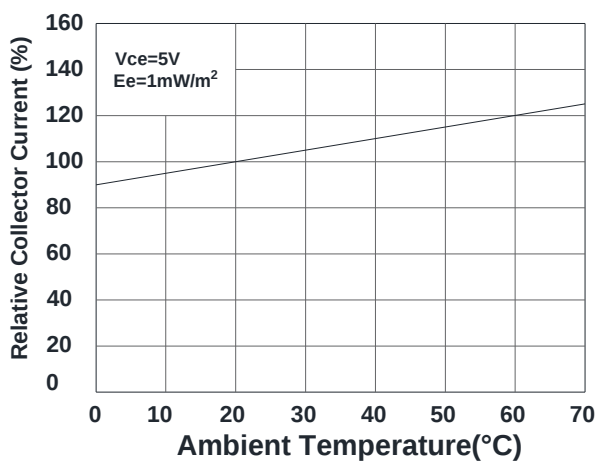
Relative Collector Current vs. Ambient Temperature
