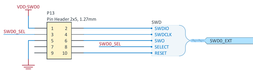
Figure 22: Debug out header
