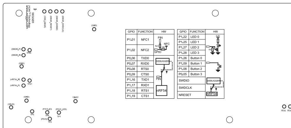
Figure 3: nRF54LM20 DK back view
