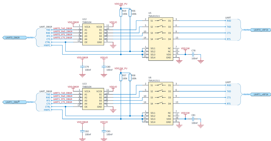
Figure 18: Analog switches between debugger and nRF54LM20B SoC
