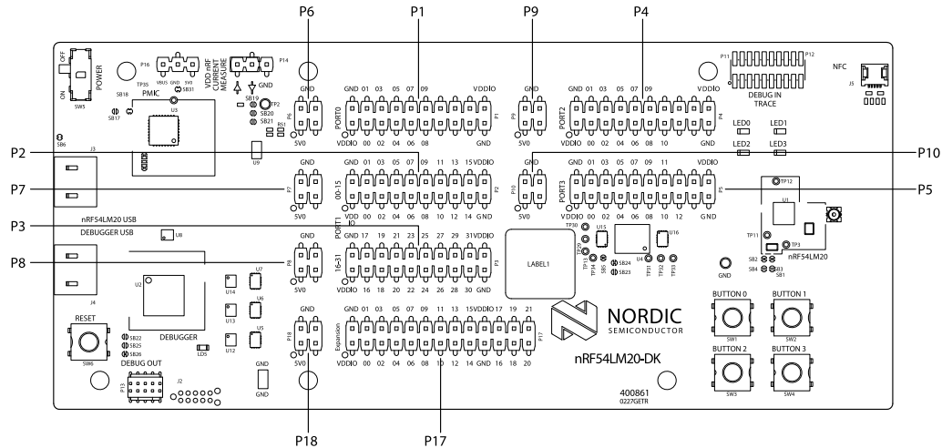
Figure 7: GPIO and power headers
