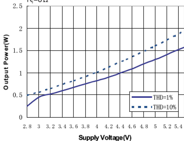
Output Power VS. Supply Voltage R_L=8\Omega
