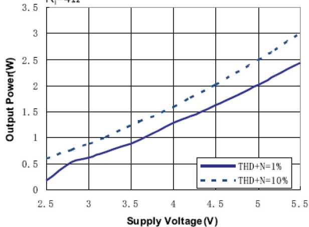
Output Power VS. Supply Voltage R_L=4\Omega
