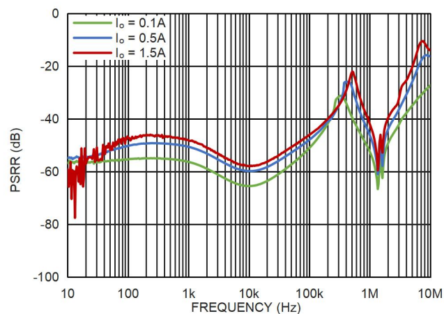
图 21. PSRR, V_{IN} = 5.3V , V_{OUT} = 5.0V
