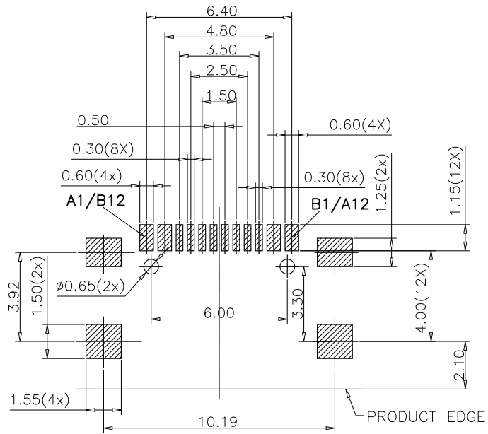
RECOMMENDED PCB LAYOUT(COMPONENT SIDE) TOLERANCE FOR PCB LAYOUT IS ±0.05
