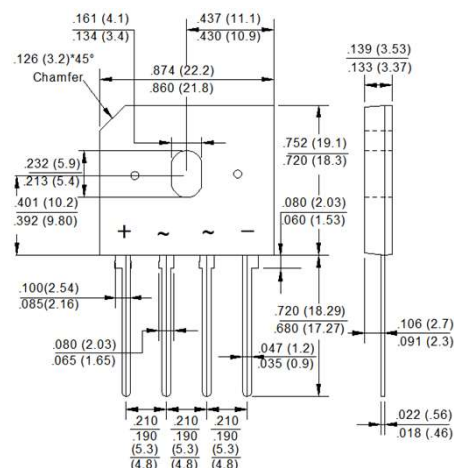
Package Outline Dimensions in Inches (Millimeters)
