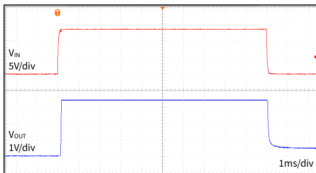
Figure 13 Line Transient
