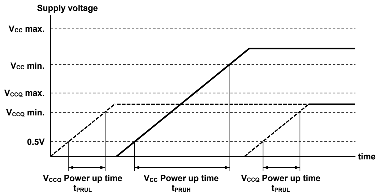
Figure 5 Power up sequence
