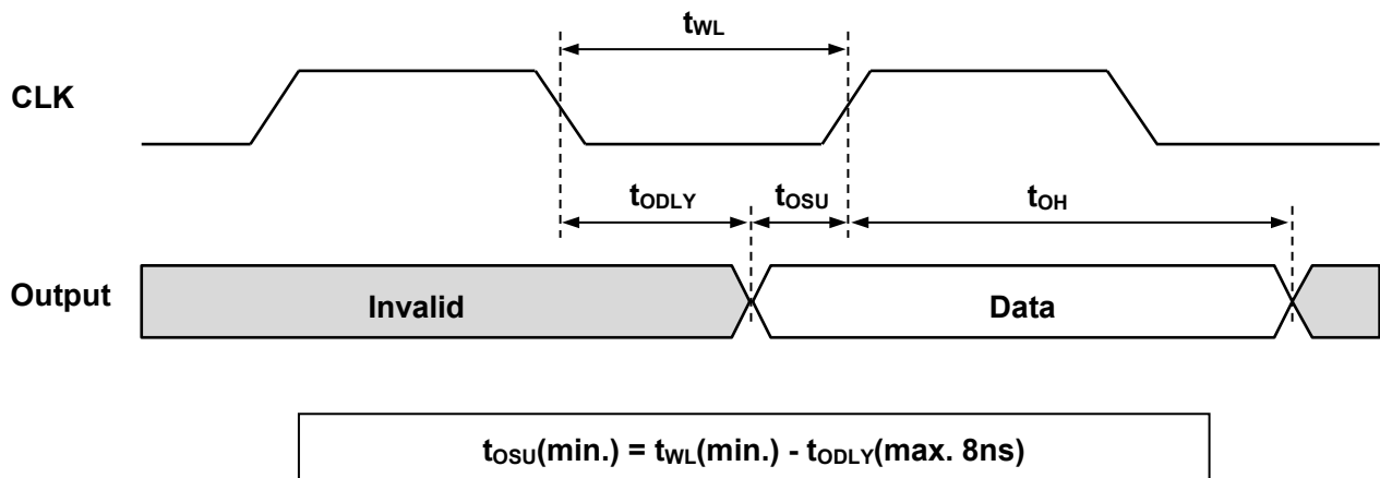
Figure 2 Output timing
