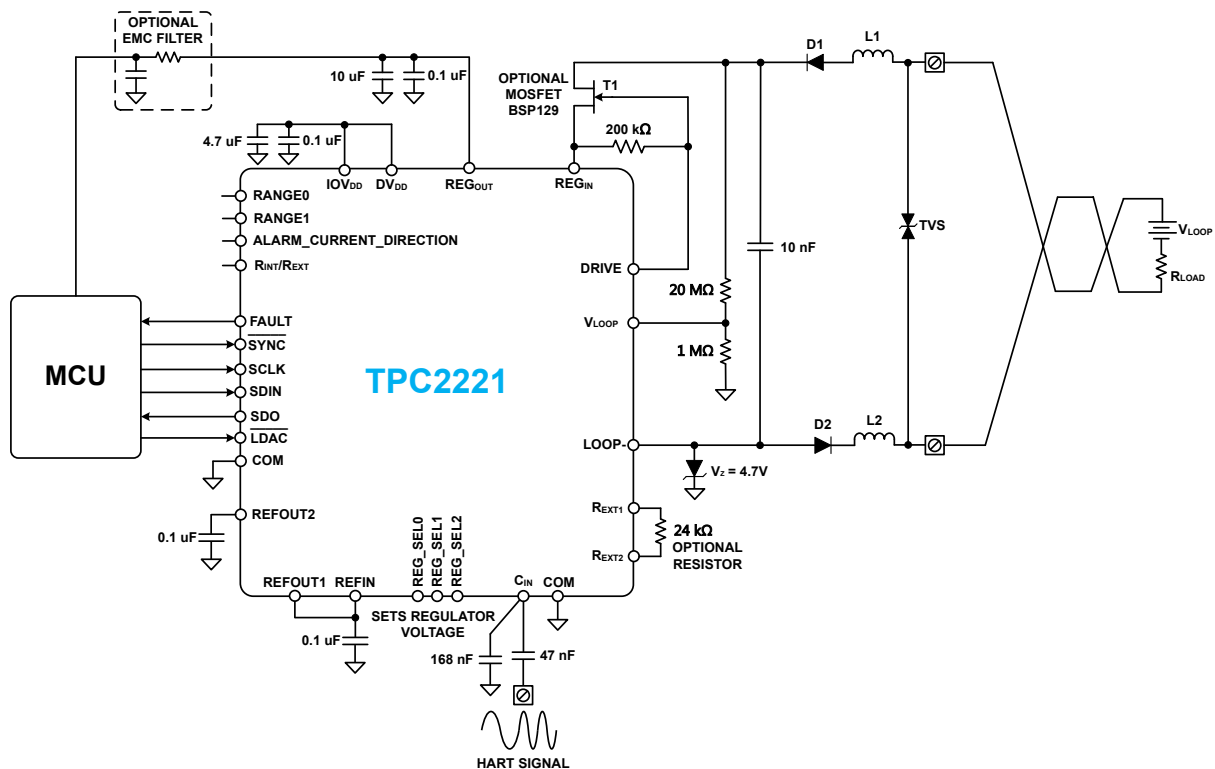
Figure 46. TPC2221 Application Diagram for HART Capable Smart Transmitter
