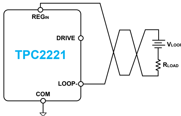
Figure 41. Direct Connection of the TPC2221 to Loop Power Supply
