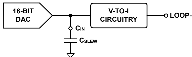
Figure 43. Slew Capacitor Circuit
