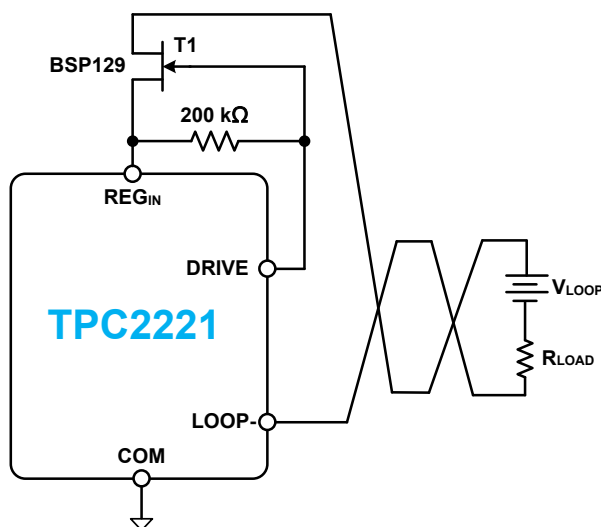
Figure 42. MOSFET Connecting the TPC2221 to Loop Power Supply
