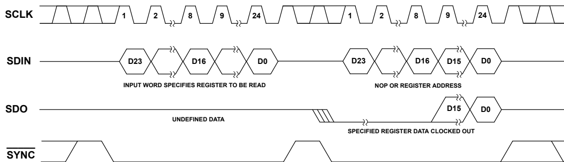
Figure 2. Readback Mode Timing Diagram
