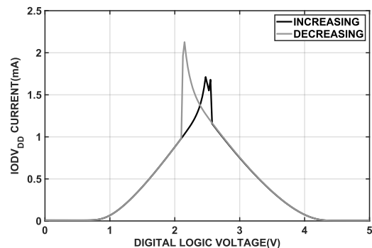
Figure 27. IODV DD Current vs. Digital Logic Voltage, Increasing and Decreasing, IODV DD = 5 V
