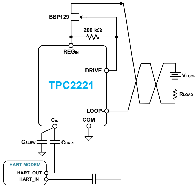
Figure 45. Connecting a HART Modem to the TPC2221
