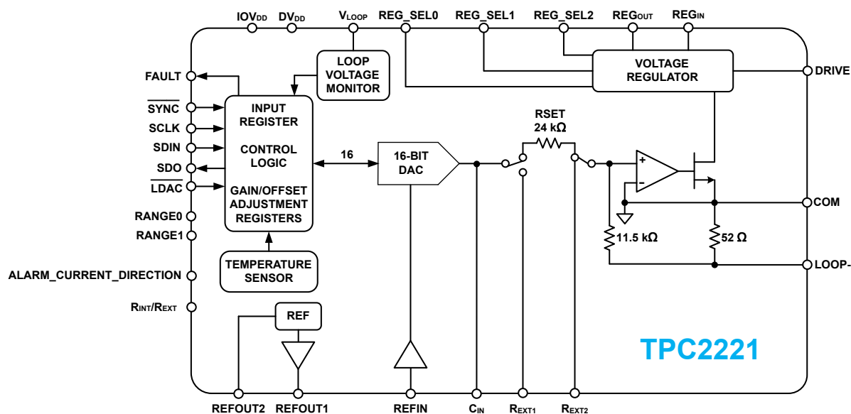
Figure 38. Functional Block Diagram
