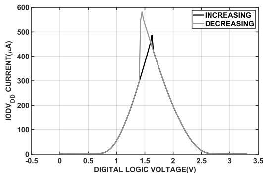
Figure 26. IODV DD Current vs. Digital Logic Voltage, Increasing and Decreasing, IODV DD = 3.3 V
