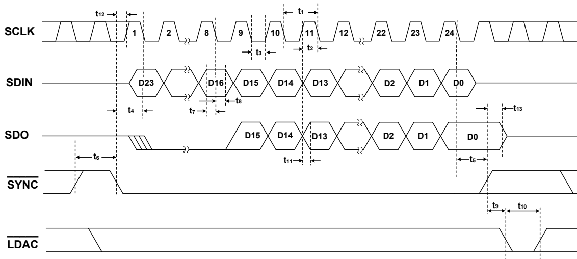
Figure 1. Write Mode Timing Diagram
