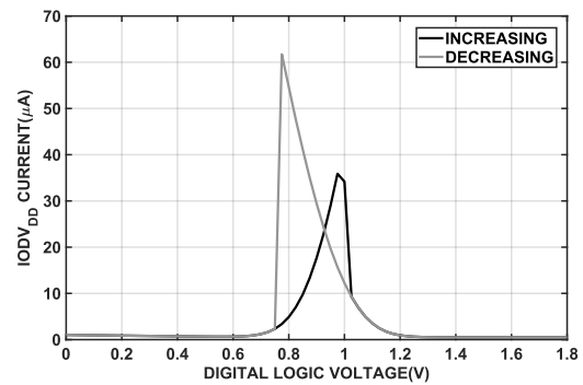
Figure 25. IODV DD Current vs. Digital Logic Voltage, Increasing and Decreasing, IODV DD = 1.8 V
