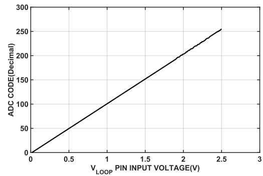
Figure 37. On-Chip ADC Code vs. V_{\text{LOOP}} Pin Input Voltage
