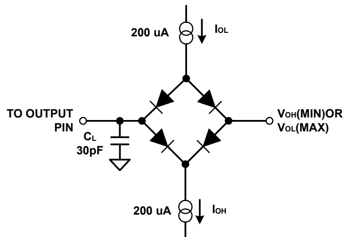
Figure 3. SDO Load Diagram
