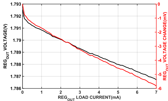
Figure 28. REG_OUT Voltage vs. Load Current
