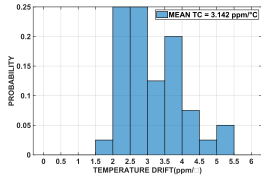
Figure 35. REFOUT1 Temperature Coefficient Histogram
