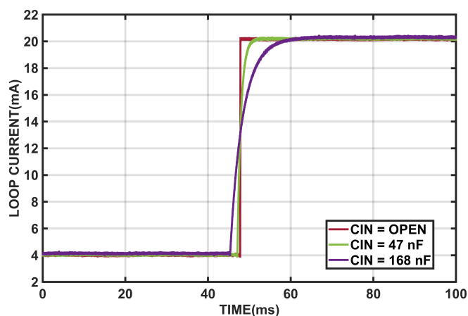
Figure 44. 4 mA to 20 mA Step with Slew Rate Control
