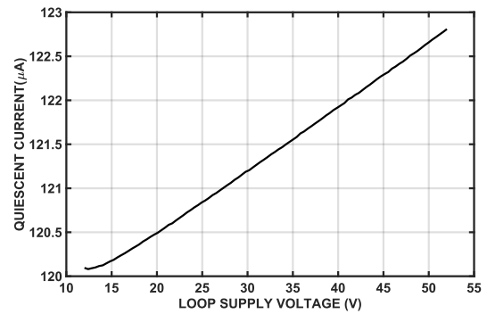
Figure 29. Quiescent Current vs. Loop Supply Voltage
