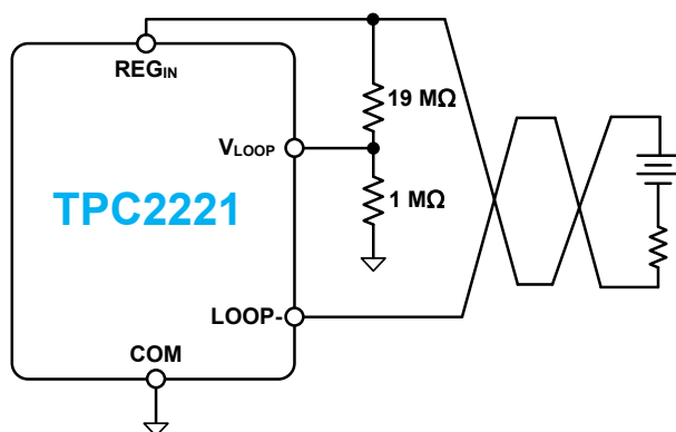
Figure 40. Resistor Divider Connection at V_{\text{LOOP}} Pin
