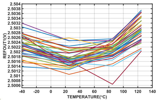
Figure 34. REFOUT1 Voltage vs. Temperature, 40 Devices Shown
