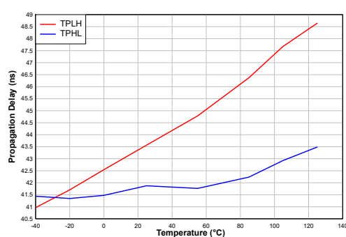
Figure 8. Output Propagation Delay vs. Temperature
