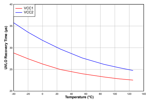
Figure 6. UVLO Recovery Time vs. Temperature
