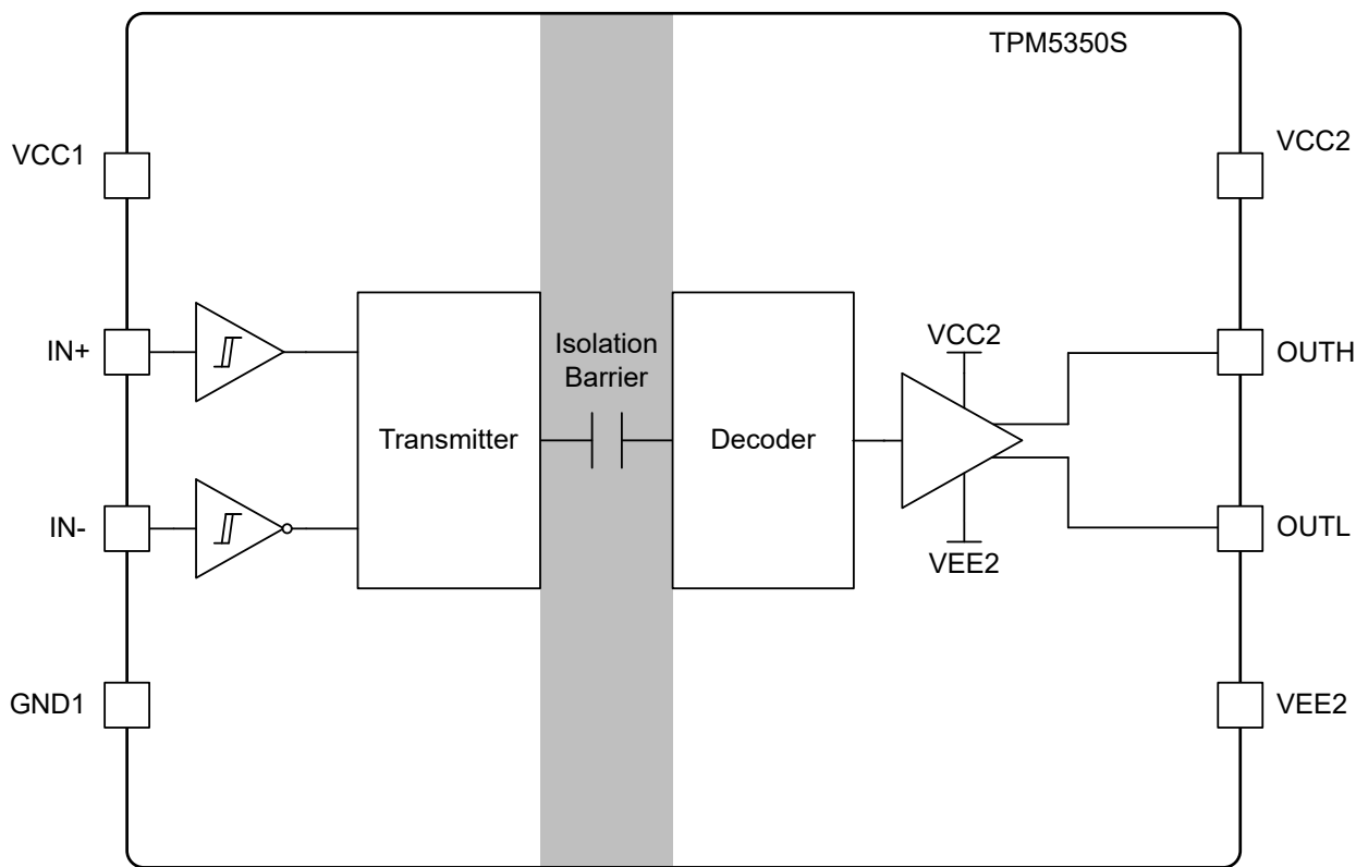
Figure 10. TPM5350S Functional Block Diagram
