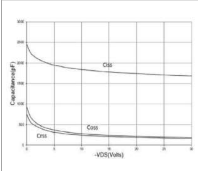
Figure 7. Capacitance Characteristics
