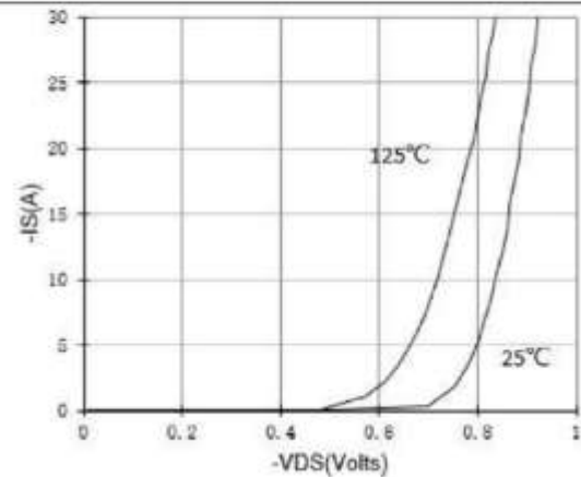
Figure 6. Body-Diode Characteristics
