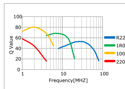
Q VALUE VS. FREQUENCY
