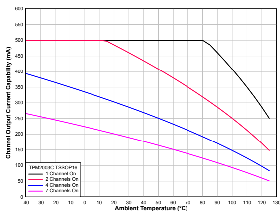
Figure 3. Output Current Capability vs. Ambient Temperature
