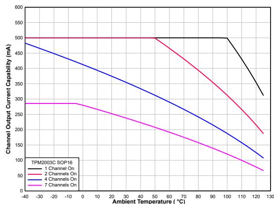
Figure 1. Output Current Capability vs. Ambient Temperature
