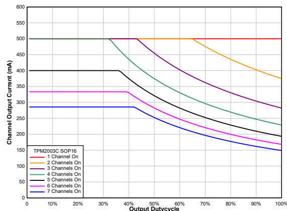
Figure 2. Output Current Capability vs. Duty Cycle,
