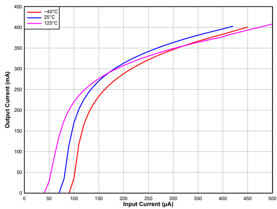
Figure 11. Output Current vs. Input Current
