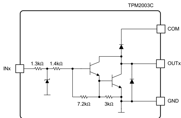
Figure 12. Functional Block Diagram
