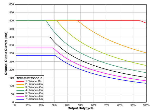
Figure 4. Output Current Capability vs. Duty Cycle
