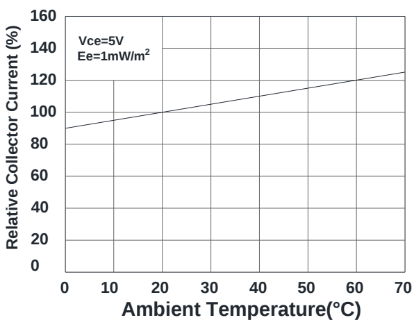
Relative Collector Current vs. Ambient Temperature
