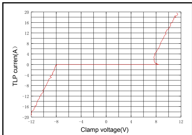
Figure 5: TLP Measurement
