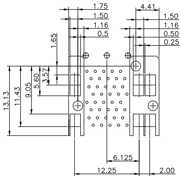
DETAIL-KEEPOUT ZONES
