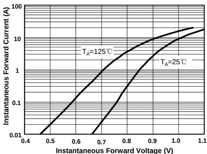
FIG.2 Typical Forward Characteristics per Diode
