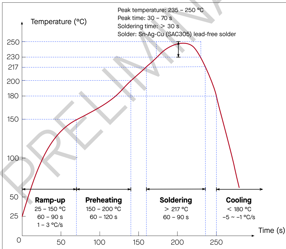
Figure 15: Reflow Profile
