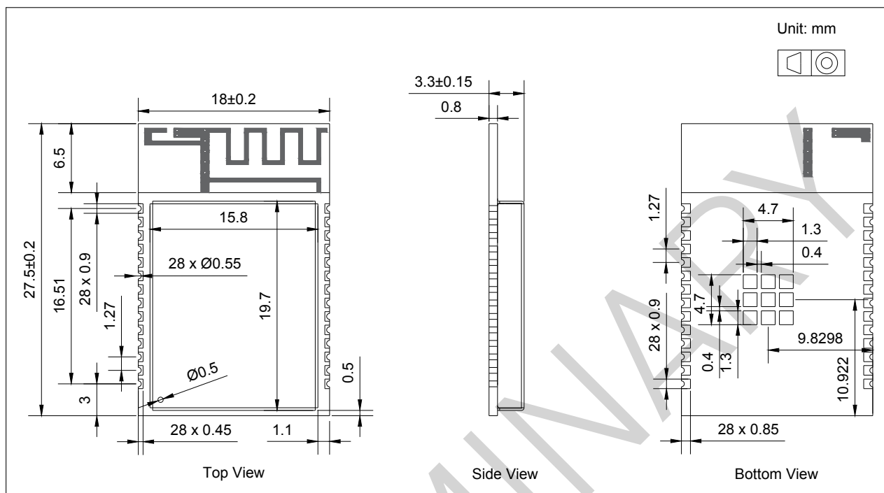
Figure 10: ESP32-C5-WROOM-1 Dimensions
