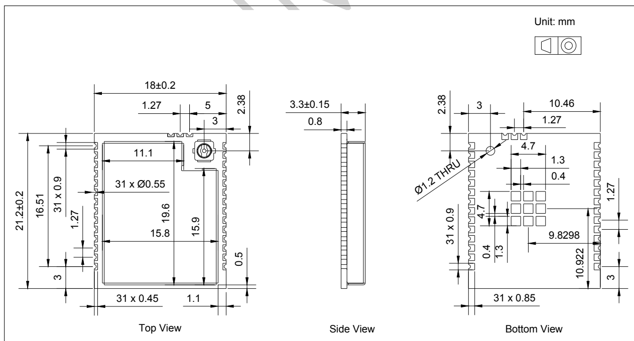
Figure 11: ESP32-C5-WROOM-1U Dimensions
