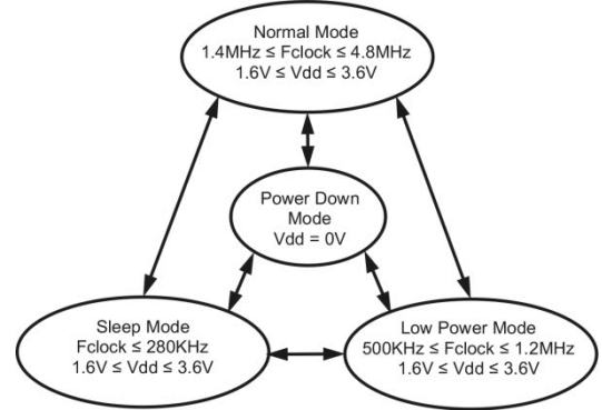
Figure 4: State Diagram
