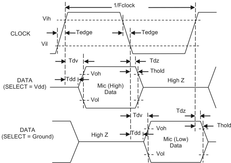
Figure 1: Timing Diagram
