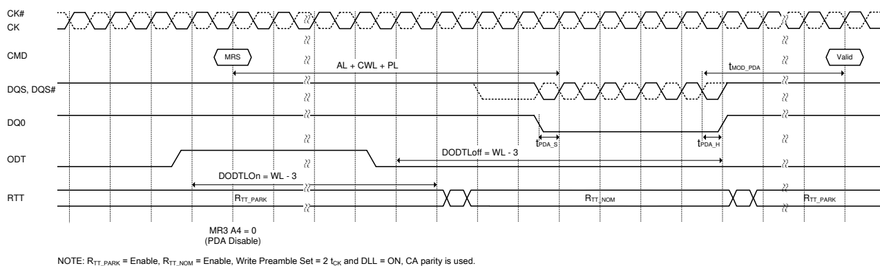
Figure 55. MRS w/ per DRAM addressability (PDA) Exit
