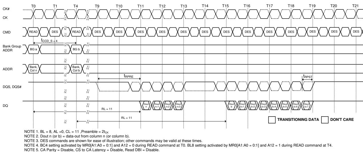
Figure 112. READ (BC4) to READ (BL8) OTF with 2t_{CK} Preamble in Different Bank Group
