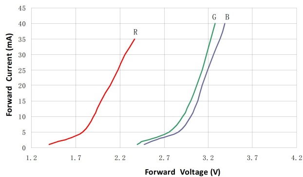
Forward Current VS. Forward Votlag (Ta=25°C)
