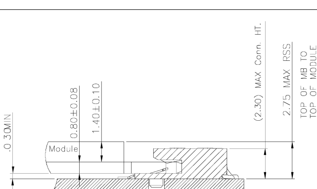
Stack-up Top Mount Single Sided Module for 1.5 max top-side component height
