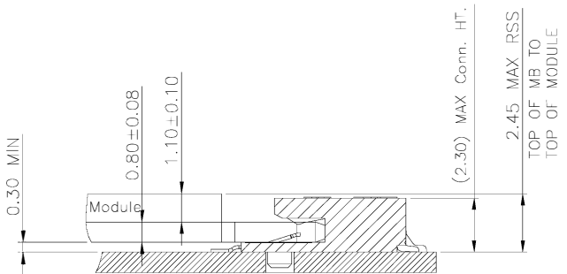
Stack-up Top Mount Single Sided Module for 1.20 max top-side component height
