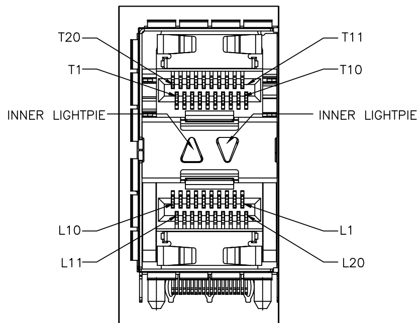
DETAIL A CIRCUIT NUMBERING AND LIGHTPIE INDENTIRCATION
