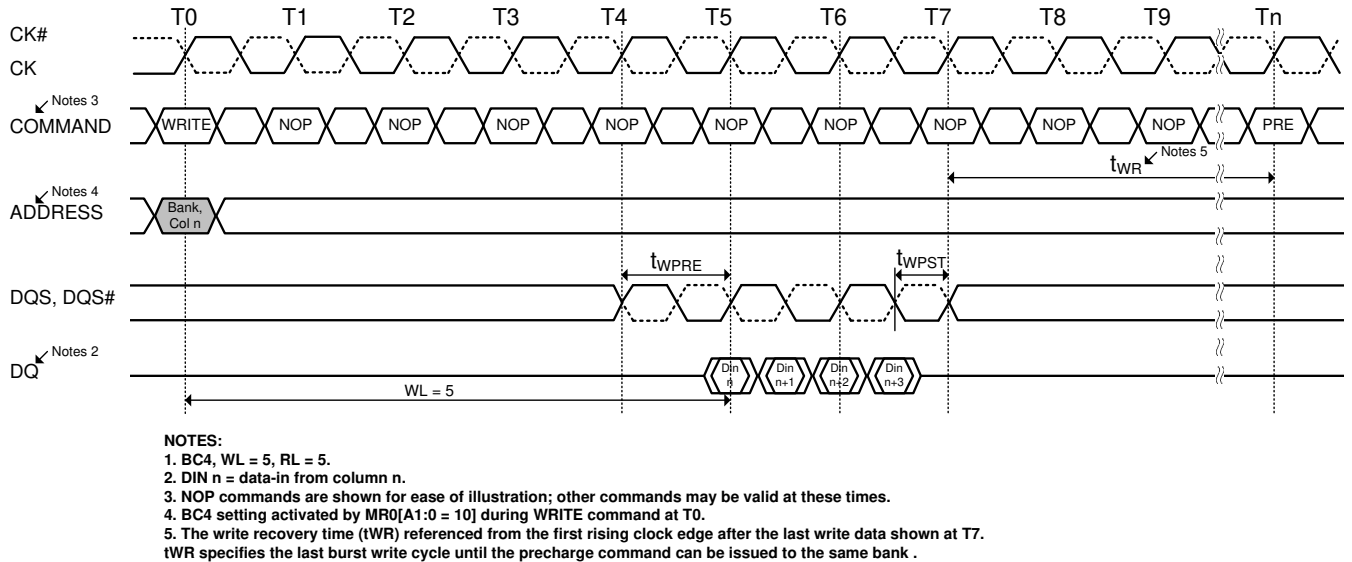
Figure 48. WRITE(BC4) to Precharge Operation
