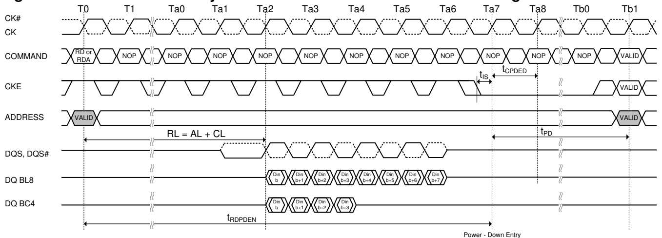
Figure 60. Power-Down Entry after Read and Read with Auto Precharge
