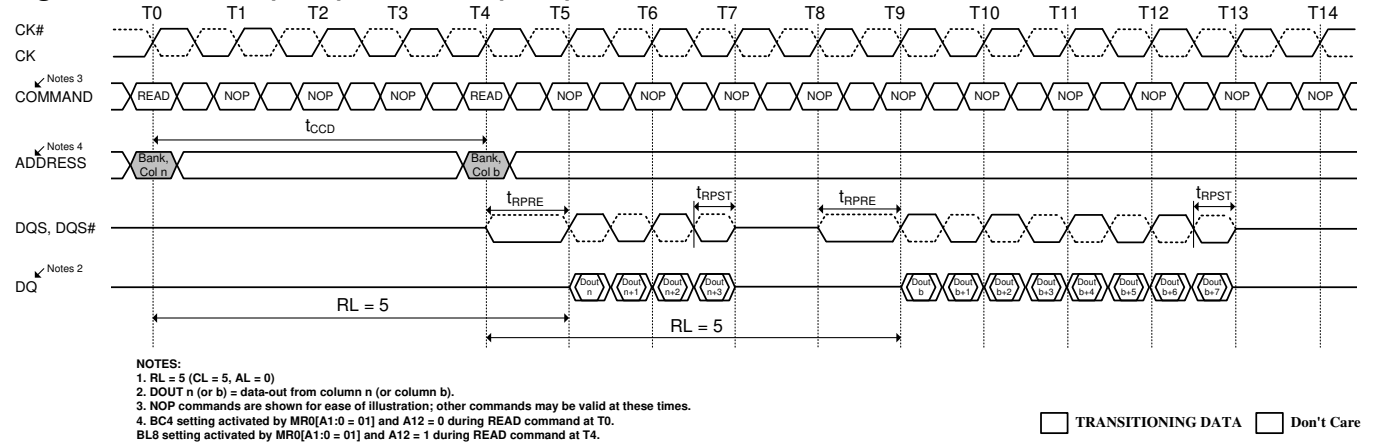
Figure 39. READ (BL4) to READ (BL8) OTF
