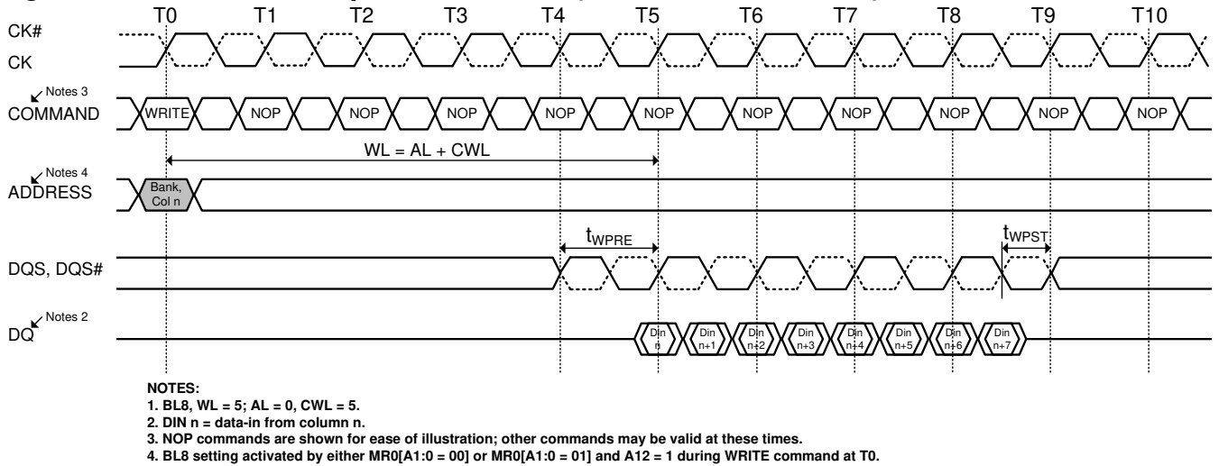
Figure 45. WRITE Burst Operation WL = 5 (AL = 0, CWL = 5, BL8)
