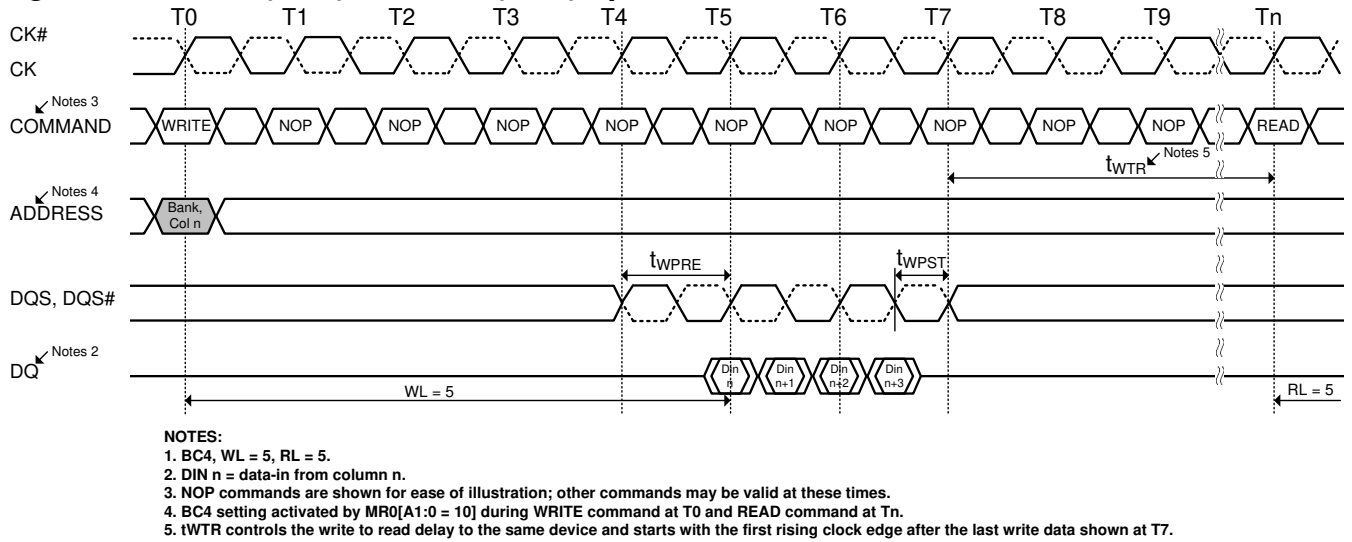
Figure 47. WRITE(BC4) to READ (BC4) operation
