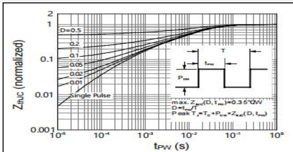
Figure 11: Normalized Transient Thermal Impedance vs Pulse Width
