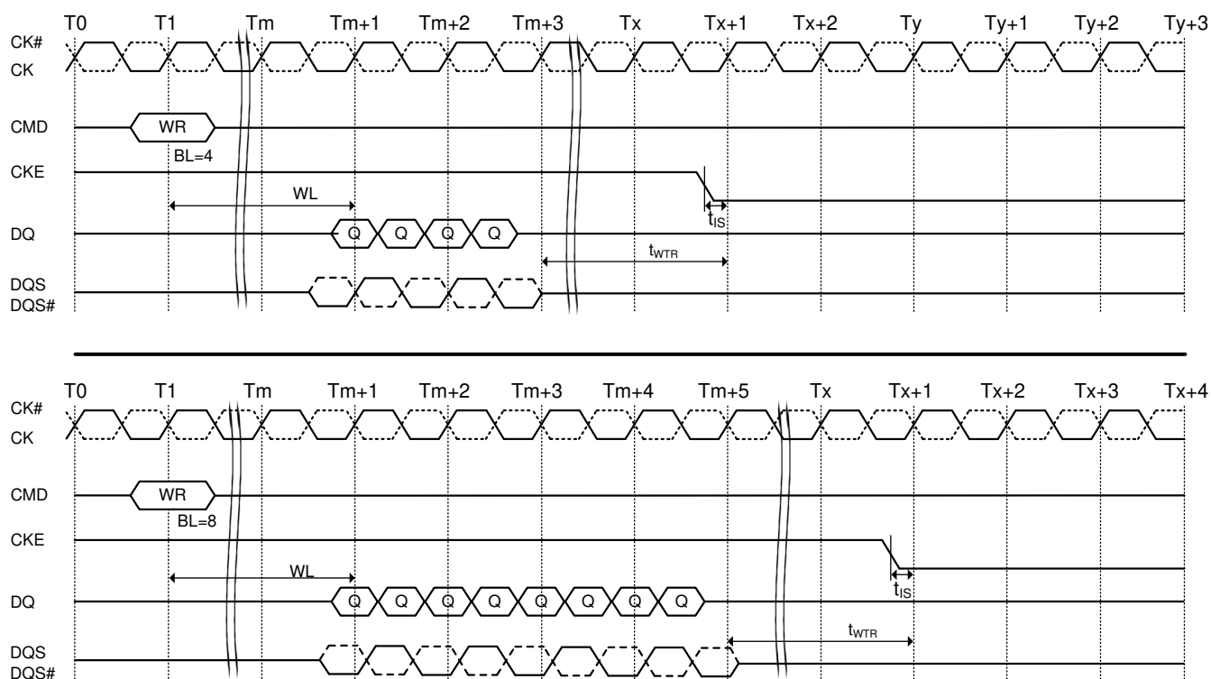
Figure 55. Write to power-down entry
