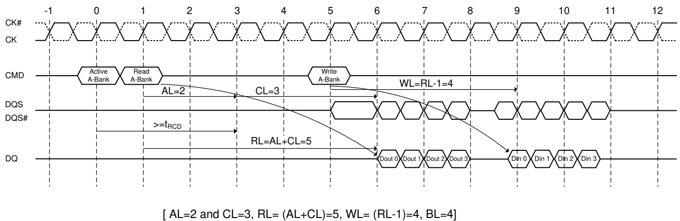
Figure 20. Posted CAS# operation: AL=2 Read followed by a write to the same bank
