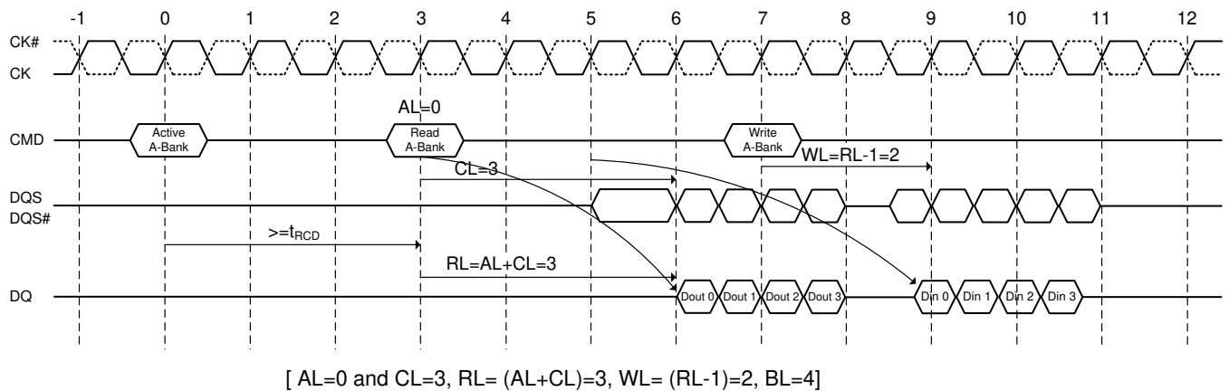
Figure 21. Posted CAS# operation: AL=0 Read followed by a write to the same bank
