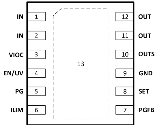
图 6. PMSOP12(4mmx4.9mm, GM12051ACPZ-1, 兼容 MSOP-12 和 DFN12 (3mmx3mm, GM12051ACPZ-4)引脚配置(顶视图)
