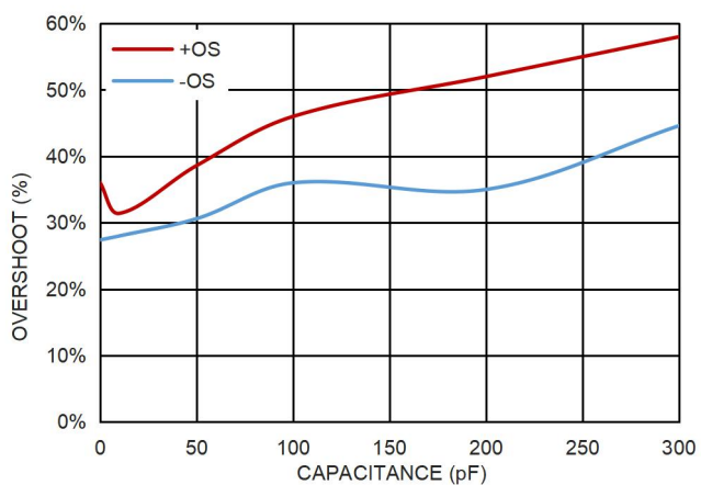
图 28. Small Signal Overshoot vs. Load Capacitance, V_S = \pm 1.35V
