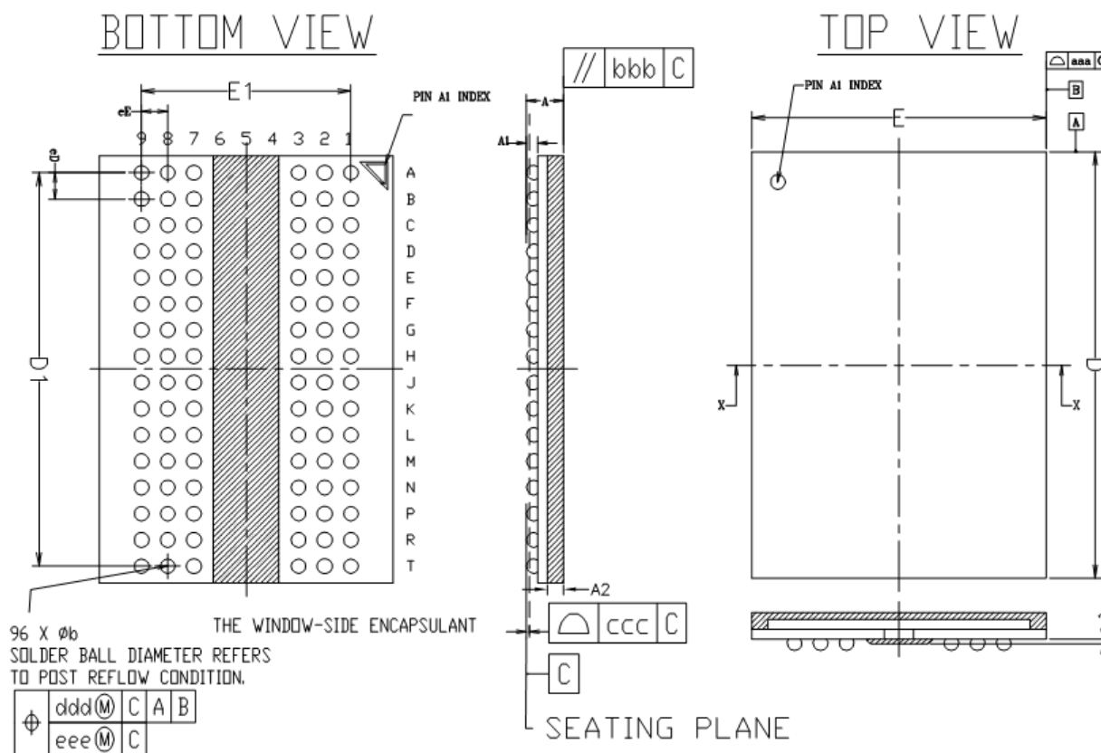
Figure 7 - Package outline for x16 component
