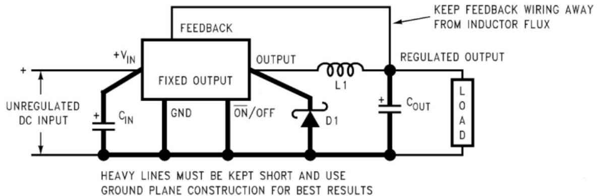
Figure 5.1. Fixed Output Voltage Version
