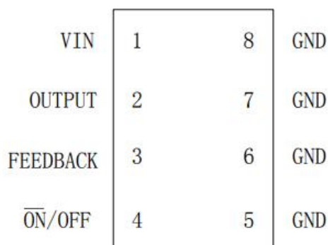
Figure 2.1: SOP8
