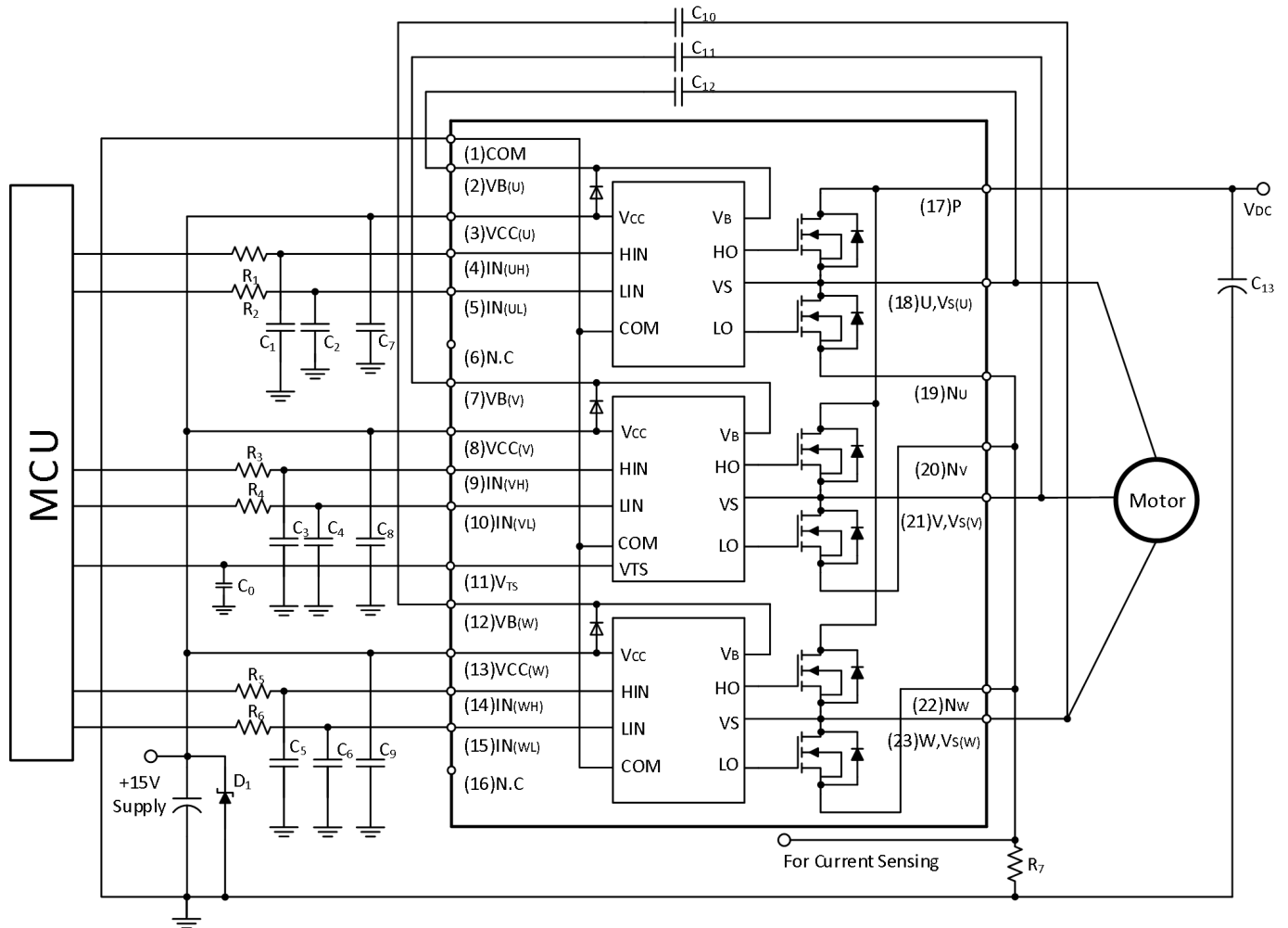
Figure8-1 Example of RC-coupling parameter 390 ohm and 1nF
