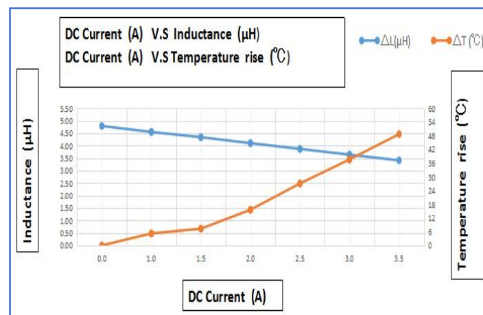
GSM0420-4R7-M
