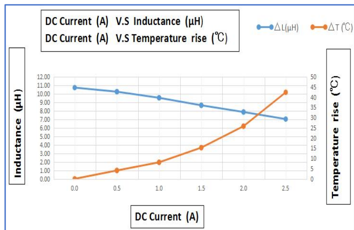
GSM0420-100-M
