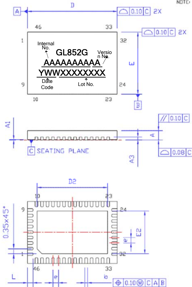
Figure 7.4 - GL852G 46 Pin LQFN Package
