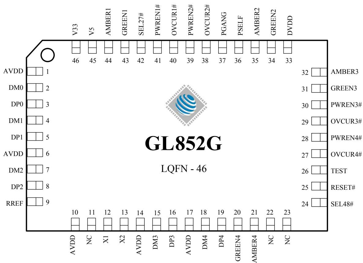
Figure 3.4 - GL852G LQFN 46 Pin Pinout Diagram
